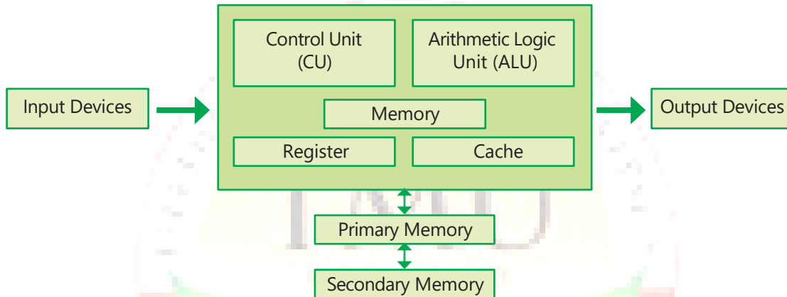
Fig. 3.3.2: Hardware Architecture
