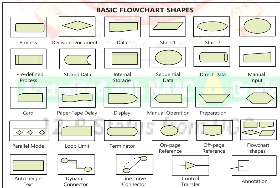
Fig. 1.7.1: Flowcharting Symbols
