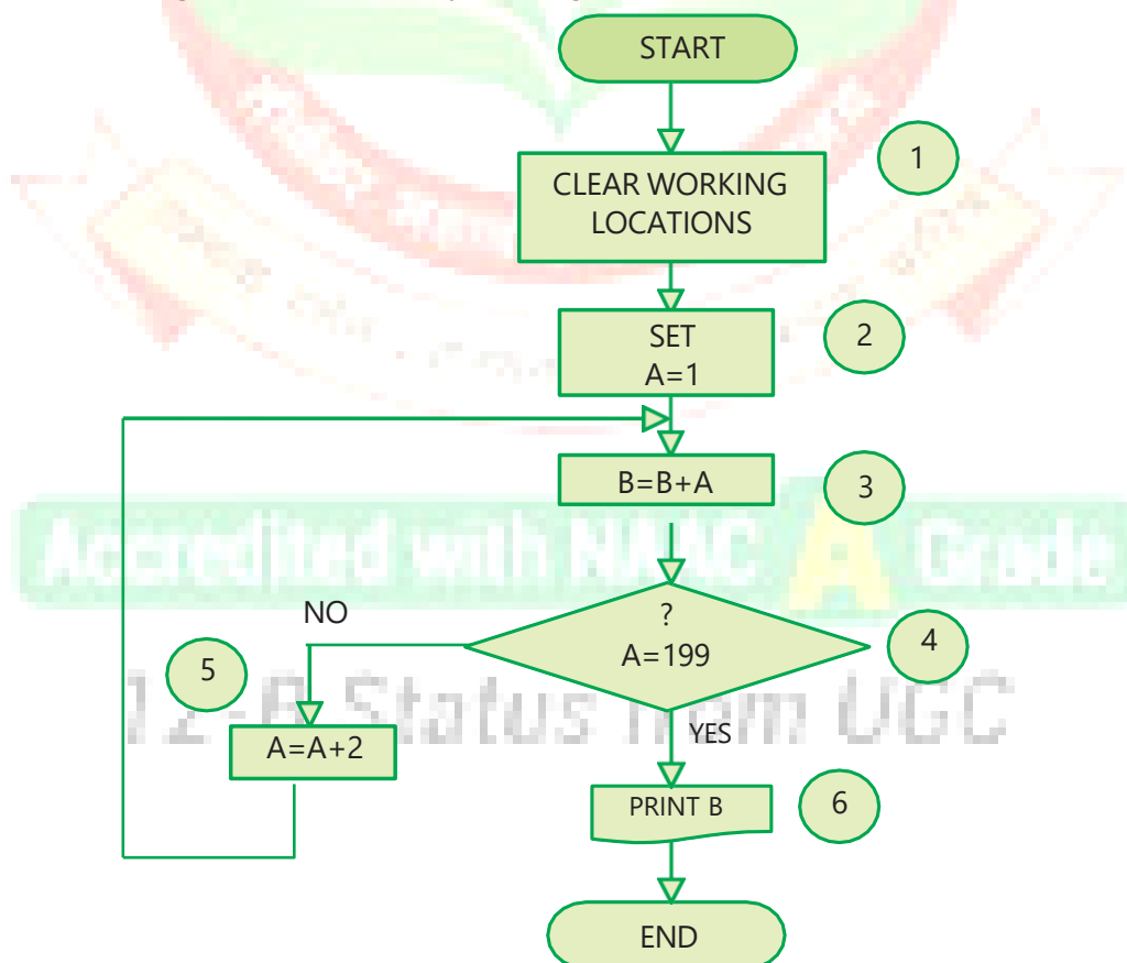
Fig. 1.7.3: Flowchart for addition of first 100 odd numbers
