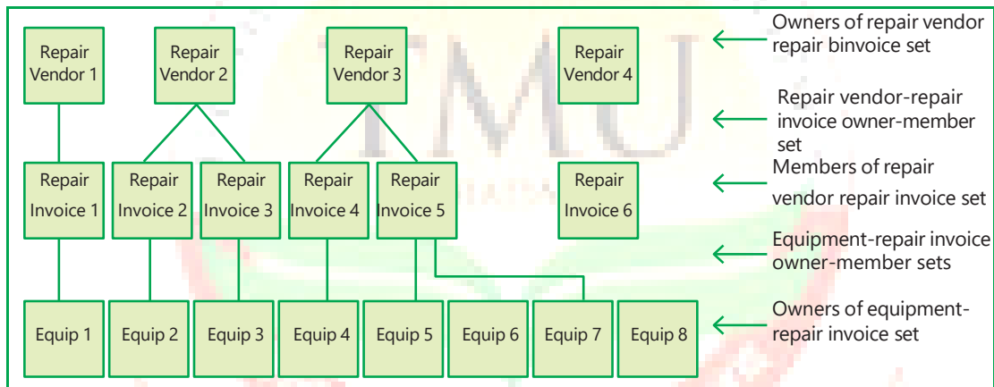
Fig. 3.3.7: Example of Network Database Model
